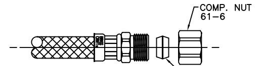
3/8 O.D. COMPRESSION OUTLET CODE: KC
